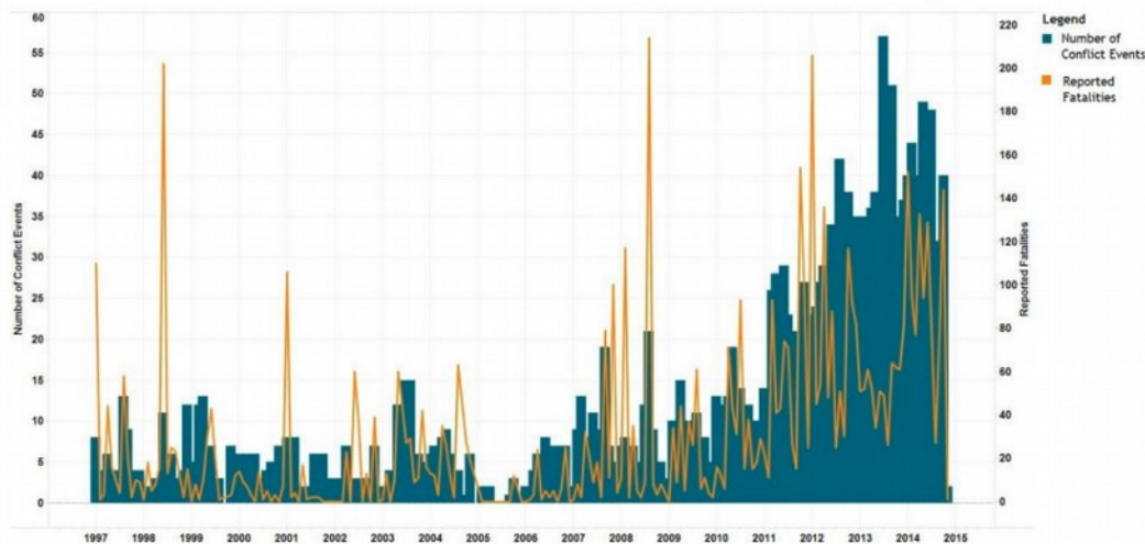
Figure 1: Number of Conflict Events and Reported Fatalities Involving IEDs, Africa, 01 January 1997-01 November 2014
