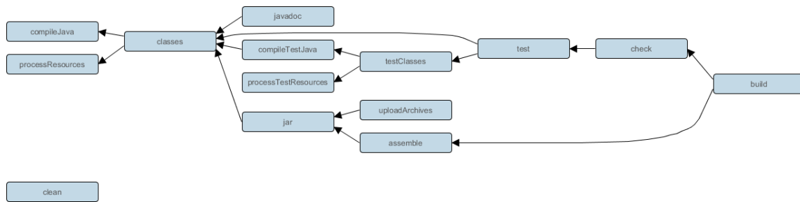
Figure 10.1. Java plugin task graph
