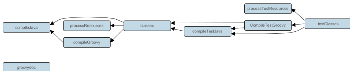
Figure 56.1. Groovy plugin - tasks
